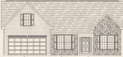
Elevation 4 with Optional Bonus Room
