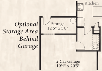
First Floor Plan - Elevations 3 & 4
