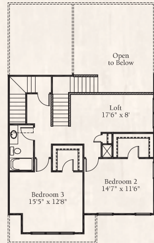
Second Floor Plan with Optional Bonus Room
